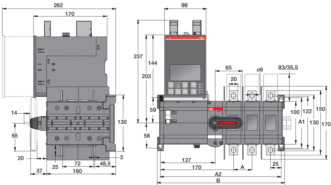
OTM160...250E_WC_8D_
