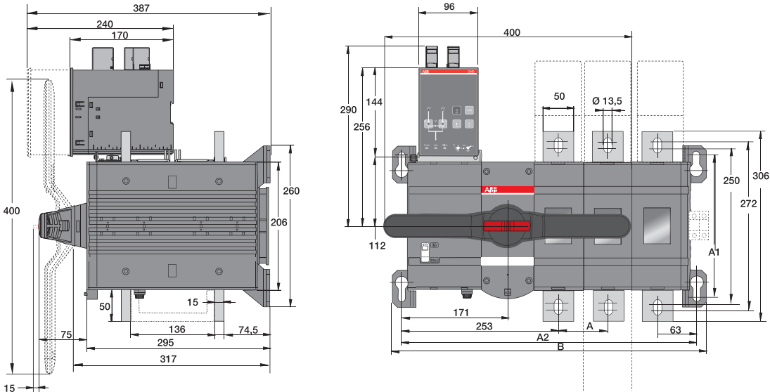
OTM1000...1250E_C2D_, OTM1000...1250E_C3D_
