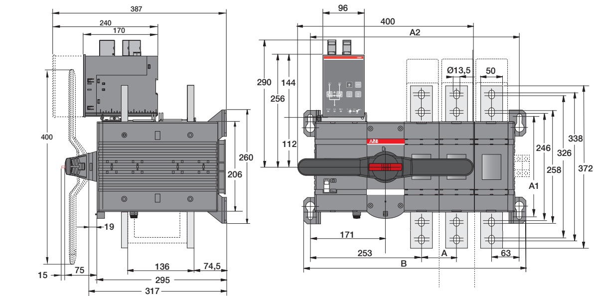
OTM1600E_C2D_, OTM1600E_C3D_
