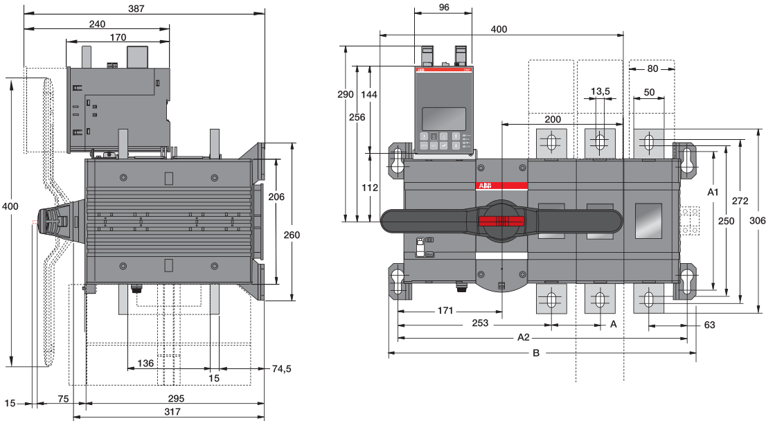
OTM1000...1250E_C_8D
