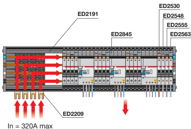
Busbar power supply from the bottom by means of 4P power supply module placed laterally
