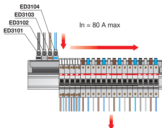
Busbar power supply by means of main row circuit-breaker fed from the top, placed laterally
