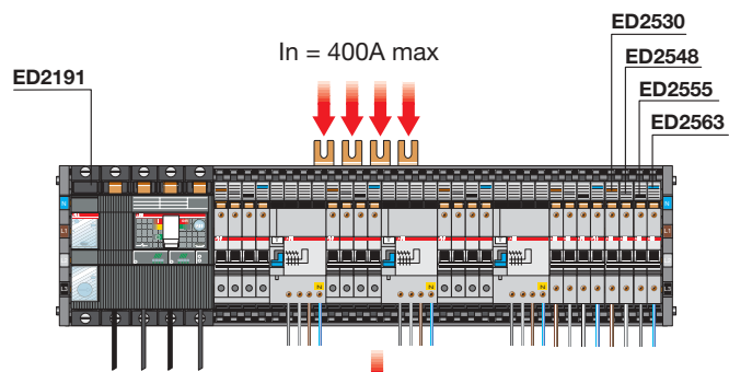
Busbar power supply from the top by means of 4P power supply module placed centrally
