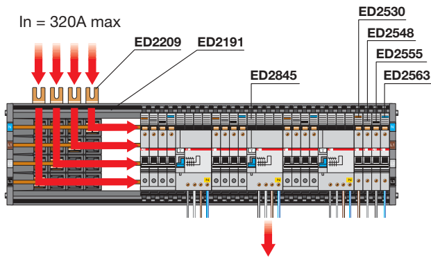
Busbar power supply from the top by means of 4P power supply module placed laterally
