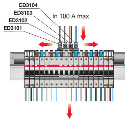
Busbar power supply by means of circuit-breaker fed from the top placed centrally
