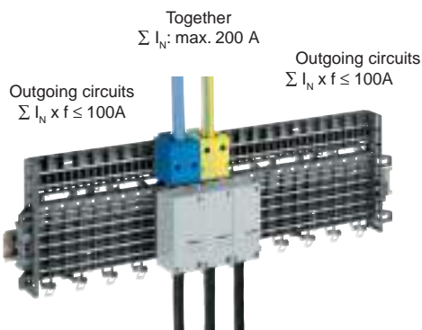
Incoming feeder, centre Upstream overcurrent protective device 200 A
